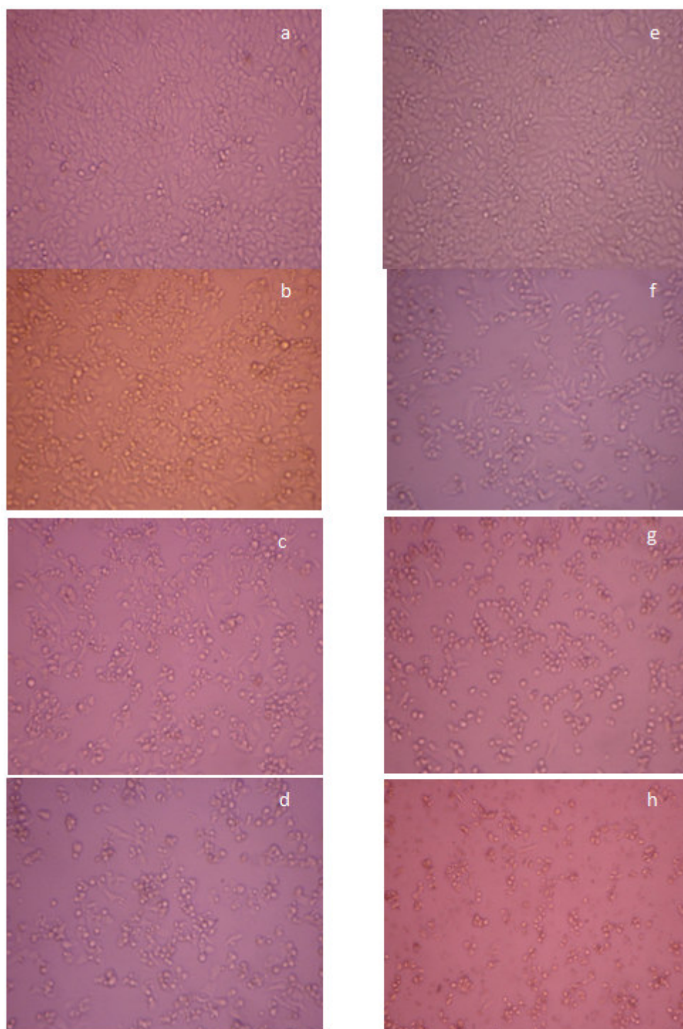
Figure 4 HeLa cell line inhibition by the sample compound (a,b,c,d) and standard drug (5-fluoro uracil) (e,f,g,h) at 0.1, 1 10 and 100μM
