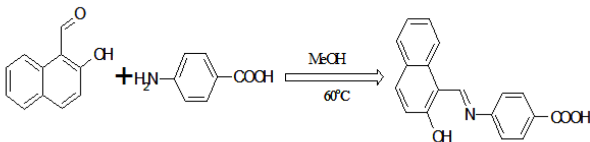
Scheme 1 Synthesis of 4-((2-hydroxynaphthalen-1-yl) methyleneamino) benzoic acid
